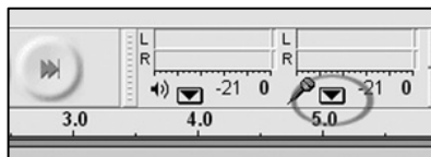
Figure 19: Monitor Input
